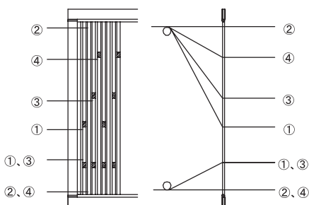
4 段綾取箄 4-way Lease Type
