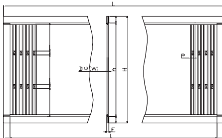
4 段綾取箄 4-way Lease Type
