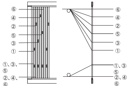
6 段綾取箄 6-way Lease Type
