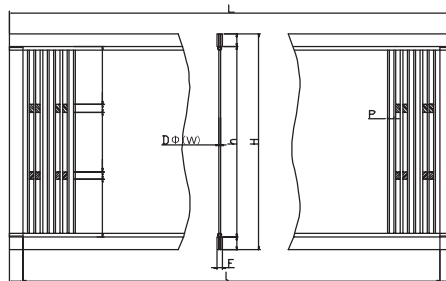
6 段綾取箄 6-way Lease Type
