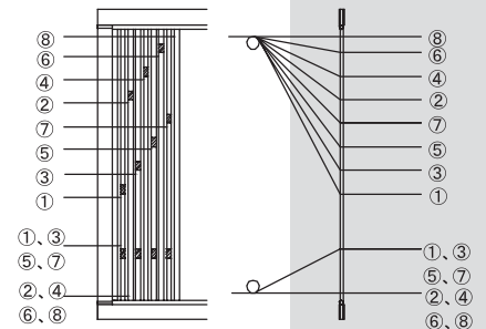
8 段綾取箄 8-way Lease Type
